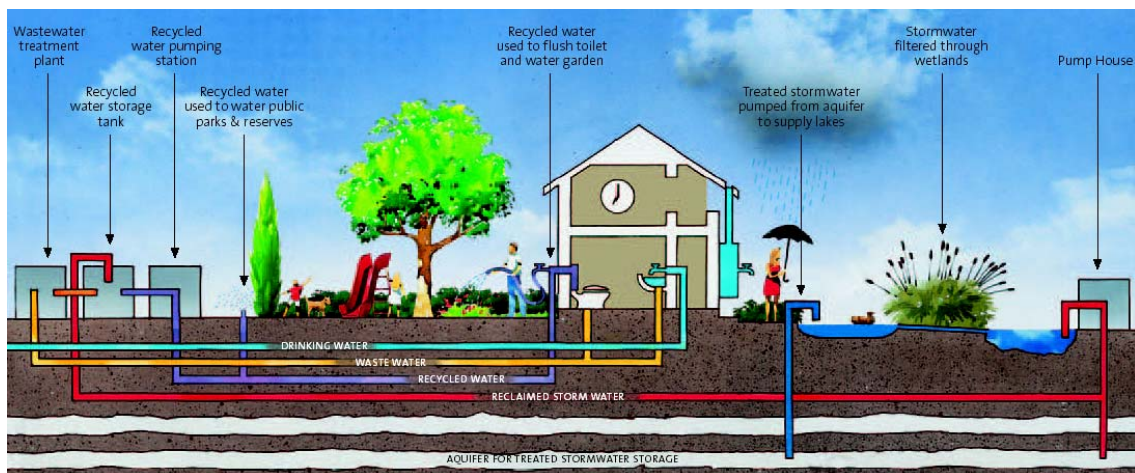
Figure 8.2 Schematic of Recycled Water Use at Mawson Lakes Residential Development
