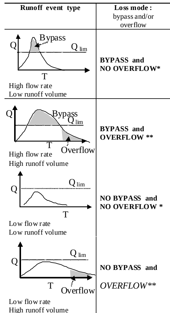
Figure A1 Hydrological Event Processes
