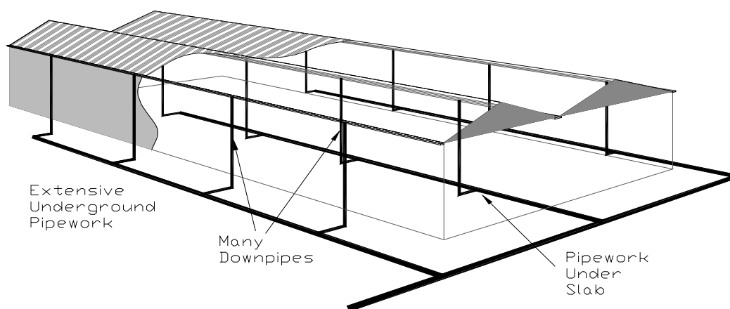
Figure 16.3: Conventional Roof Drainage System
