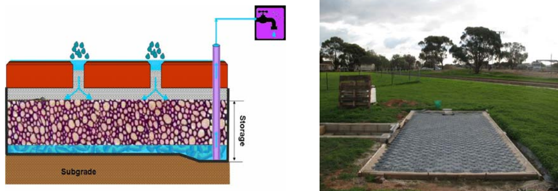
Figure 7.3 Water harvesting and reuse in a permeable pavement system at the University of South Australia
