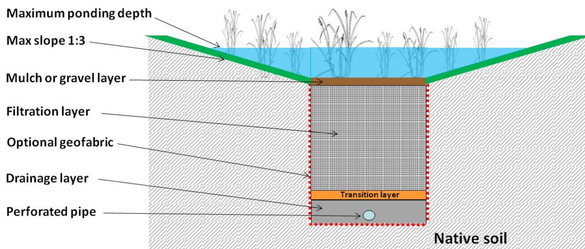
Figure 10.1 Cross Section through a Bioretention Swale
