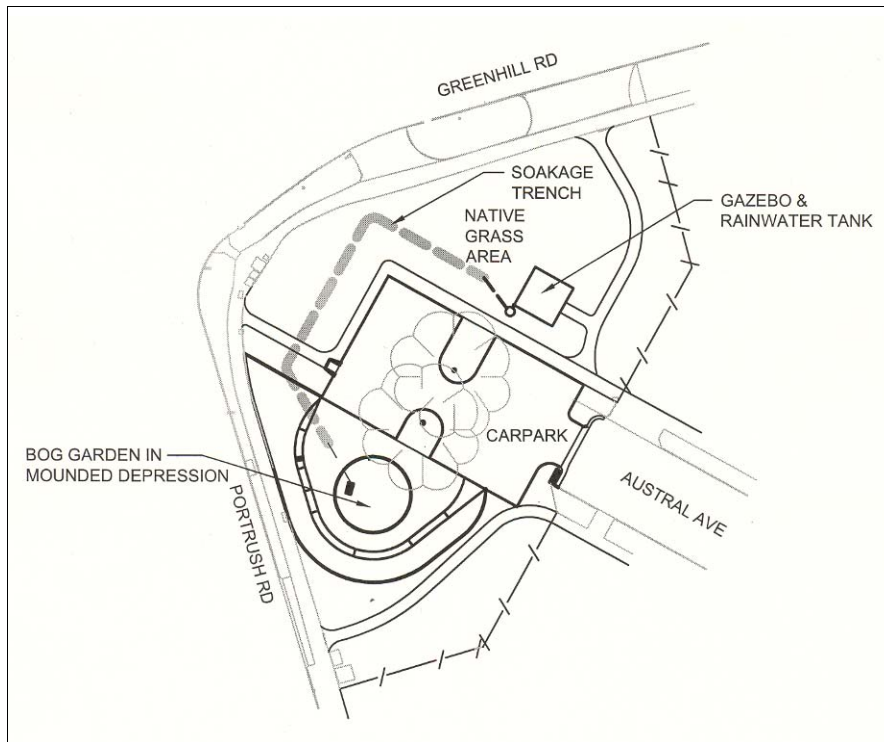
Figure 7.6 Location Plan of the Pervious Pavements, Linden Gardens
