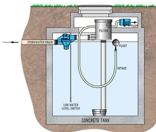
Figure 16.17: Schematic Diagram Showing Components of an ecoRain Underground Rainwater Tank
