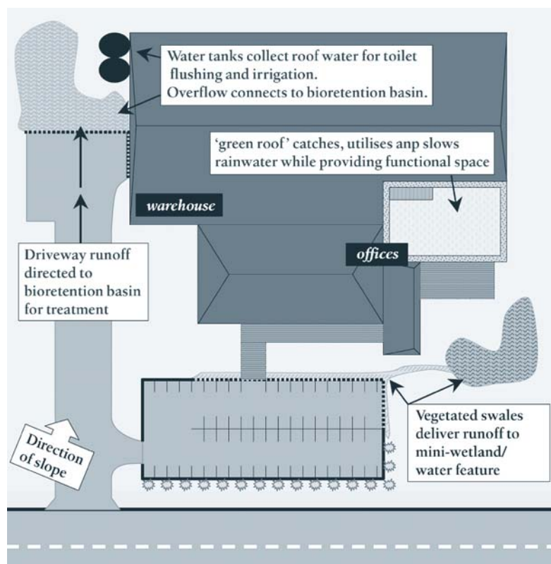
Figure 2.10 Industrial or Commercial Site Layout Example Incorporating WSUD Measures
