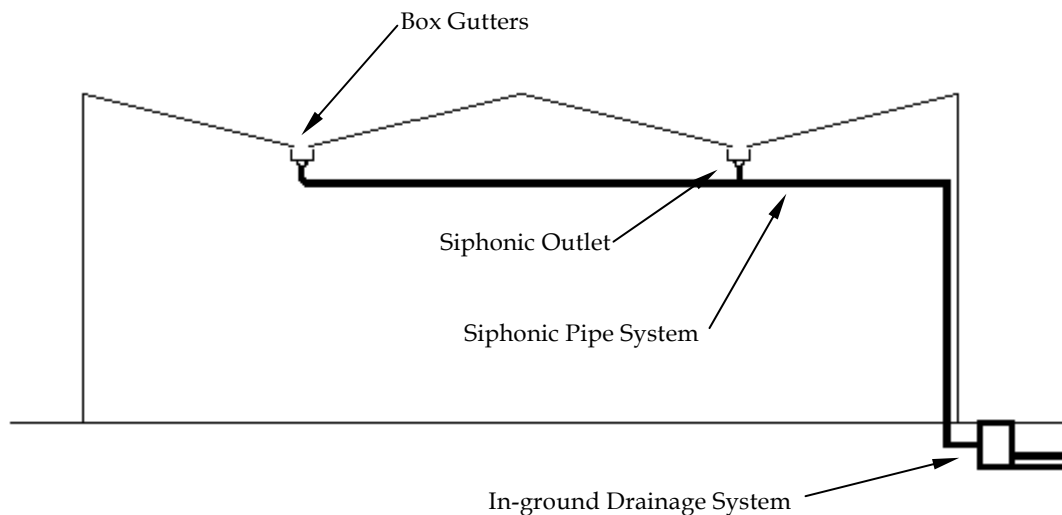
Figure 16.5: Siphonic Drainage System Components
