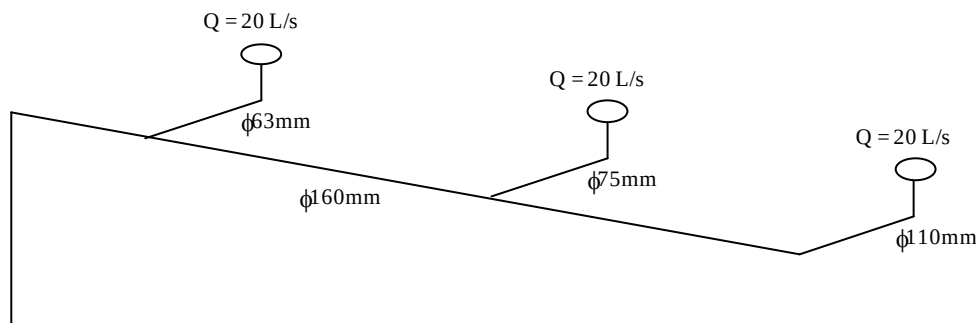
Figure 16.14: Balanced System Using Different Tailpipe Sizes
