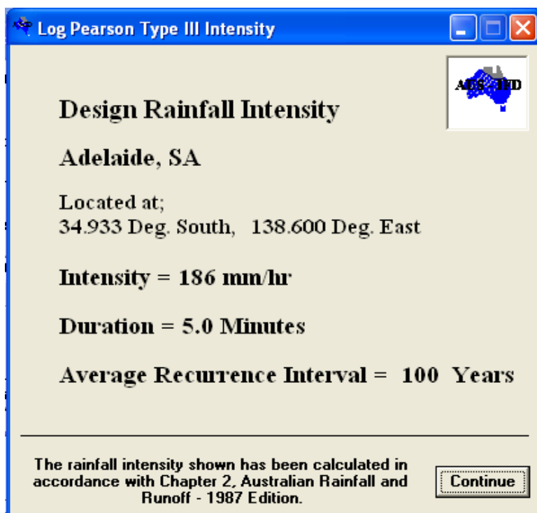
Figure 16.8: Example Output from AUS-IFD Version 2.0
