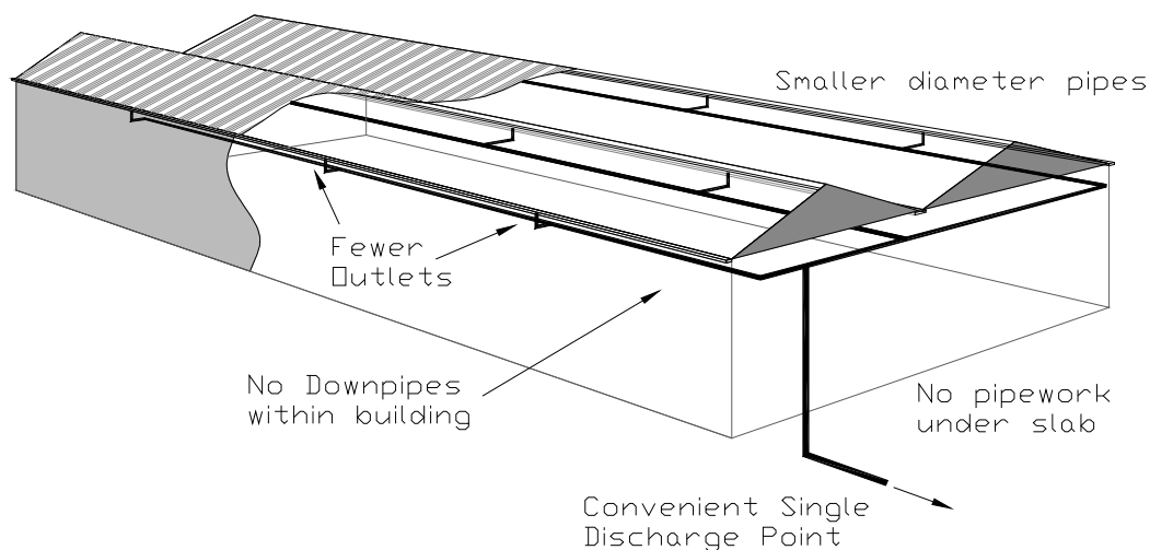
Figure 16.4 Siphonic Roof Drainage System
