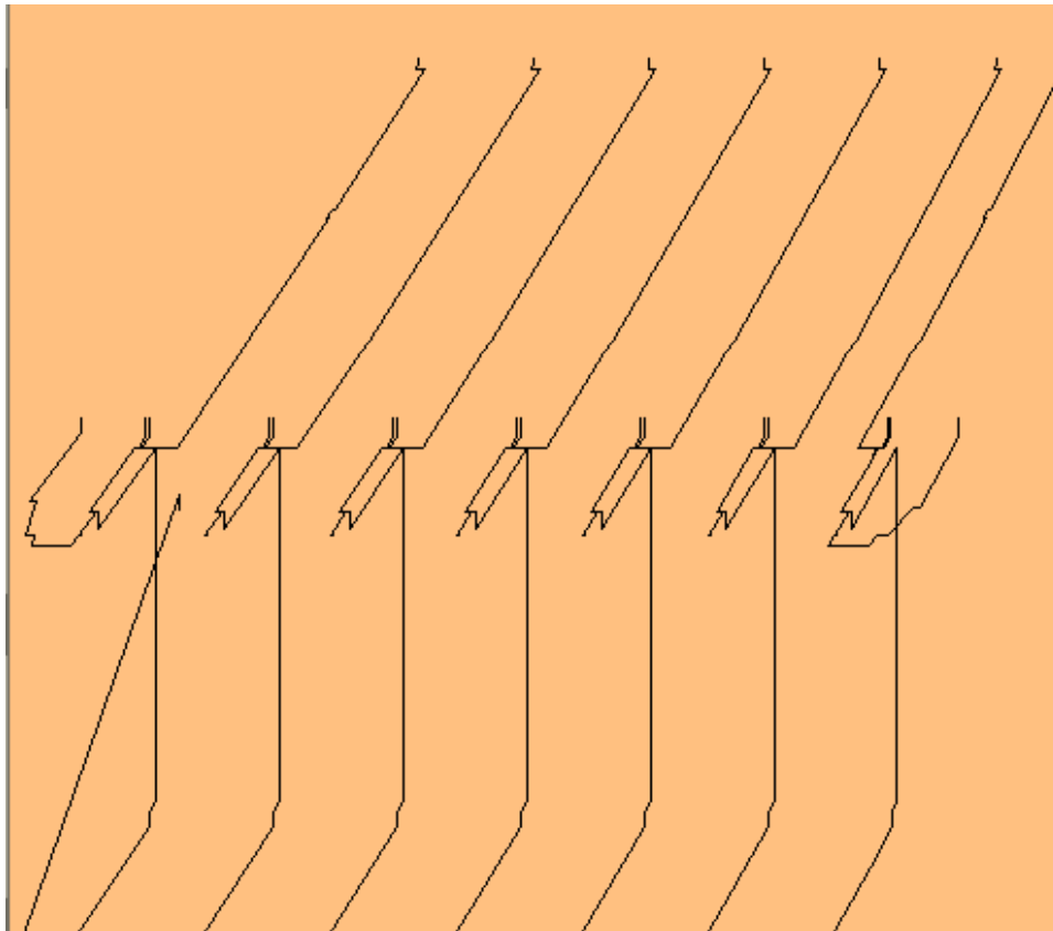
Figure 16.12: Schematic of Siphonic Pipe Layout at Adelaide Airport
