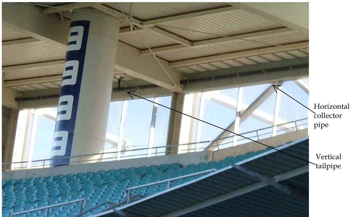
Figure 16.6: Horizontal Collector Pipe at AAMI Stadium in Adelaide
