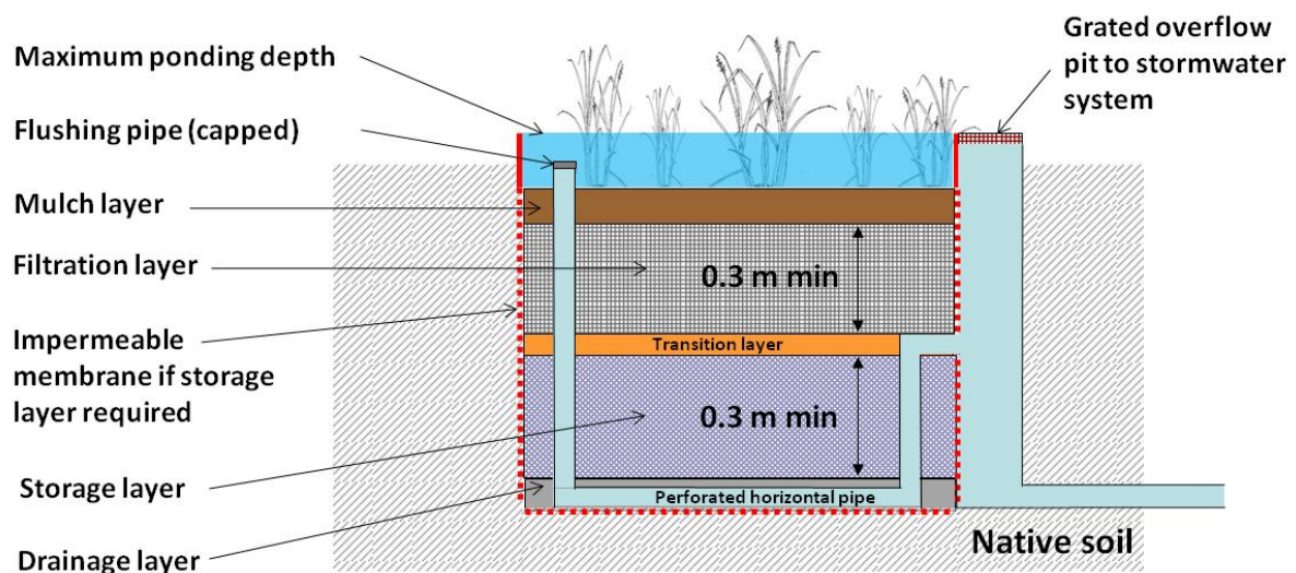
Figure 10.3 Bioretention Basin (incorporating Underground Storage Layer)
