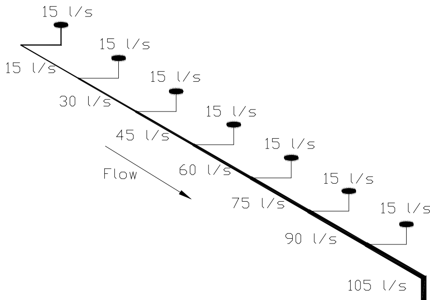
Figure 16.11: Ideal Flow Volumes in an Example System
