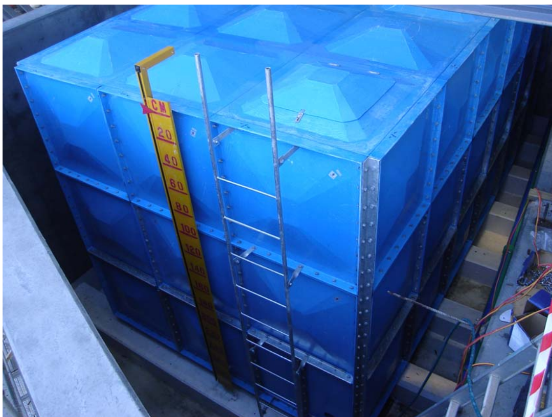
Figure 16.15: In-building Rainwater Tank Installed at the Sydney Cricket Ground
